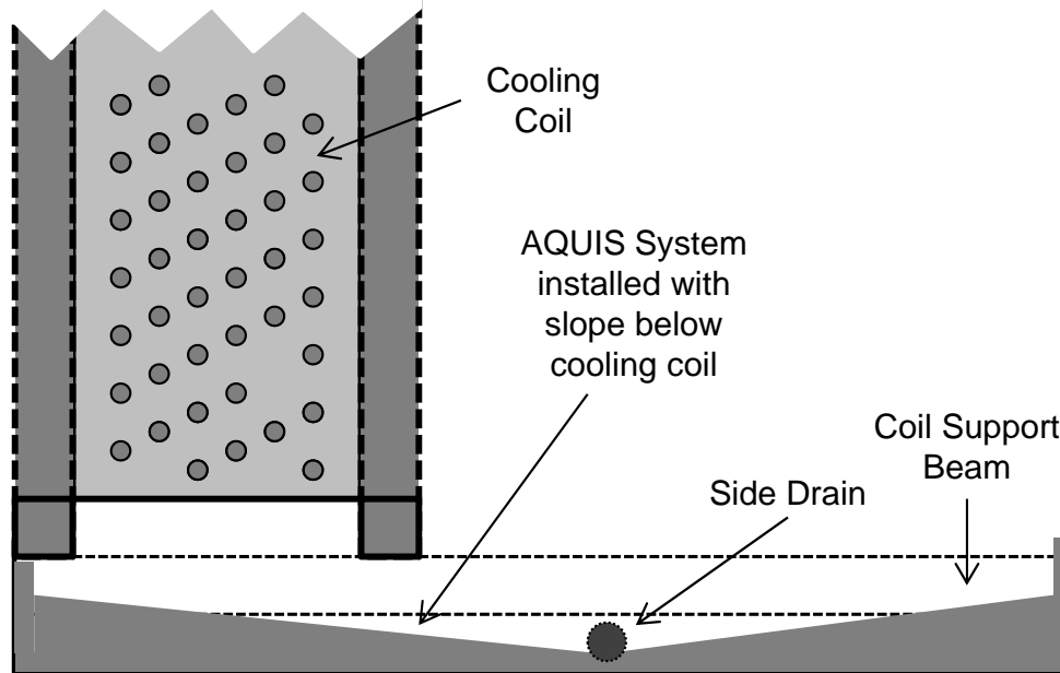
Drain Pan Side View
