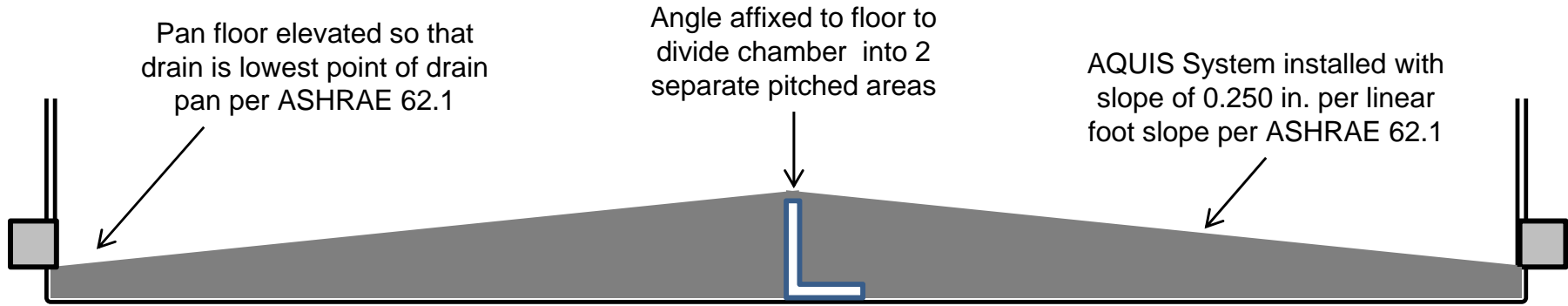
Drain Pan Front View
