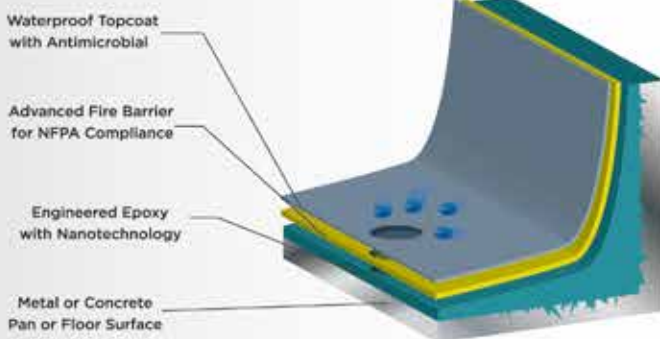
AQUIS SYSTEM DIAGRAM
